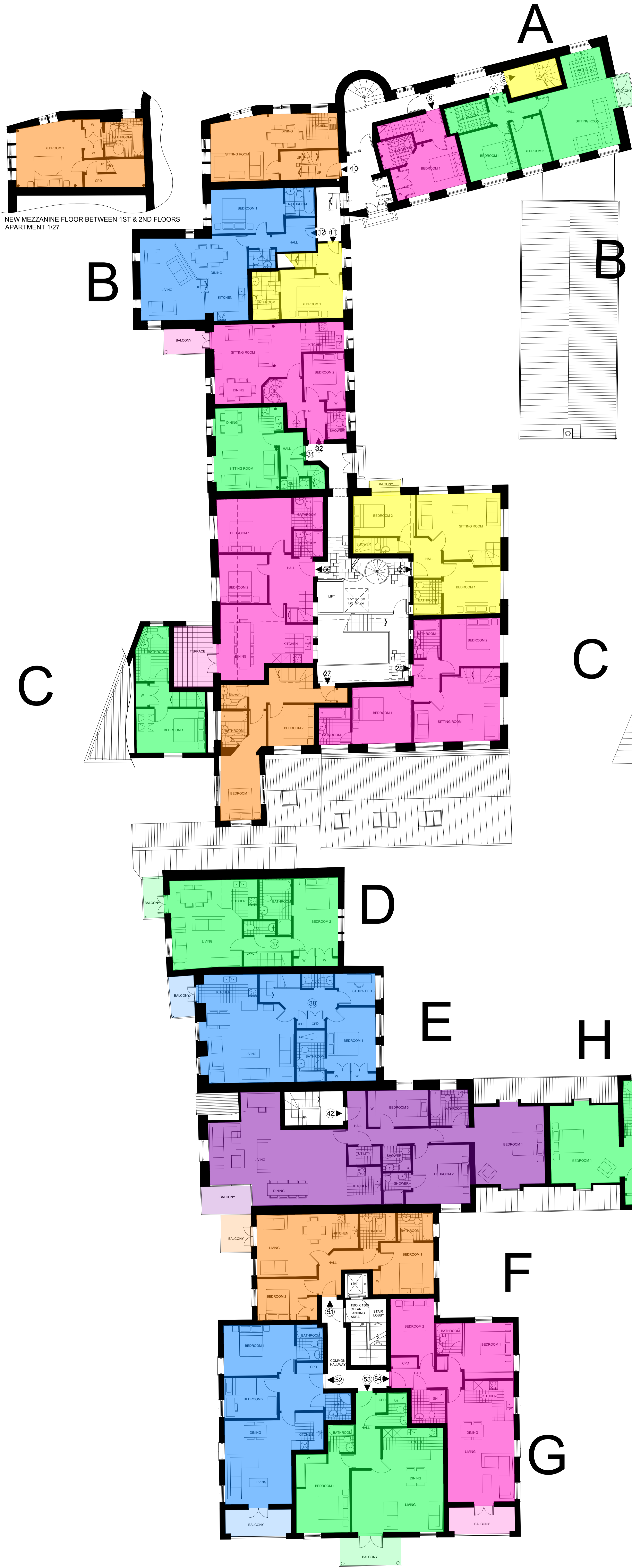
BLOCKS A - G 2ND FLOOR PLAN
